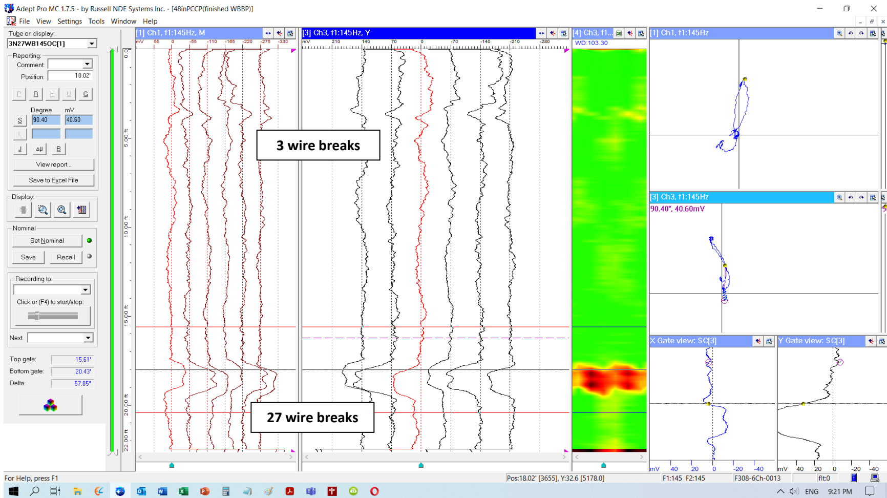
Wire-break detection in a 48" embedded concrete pipe
